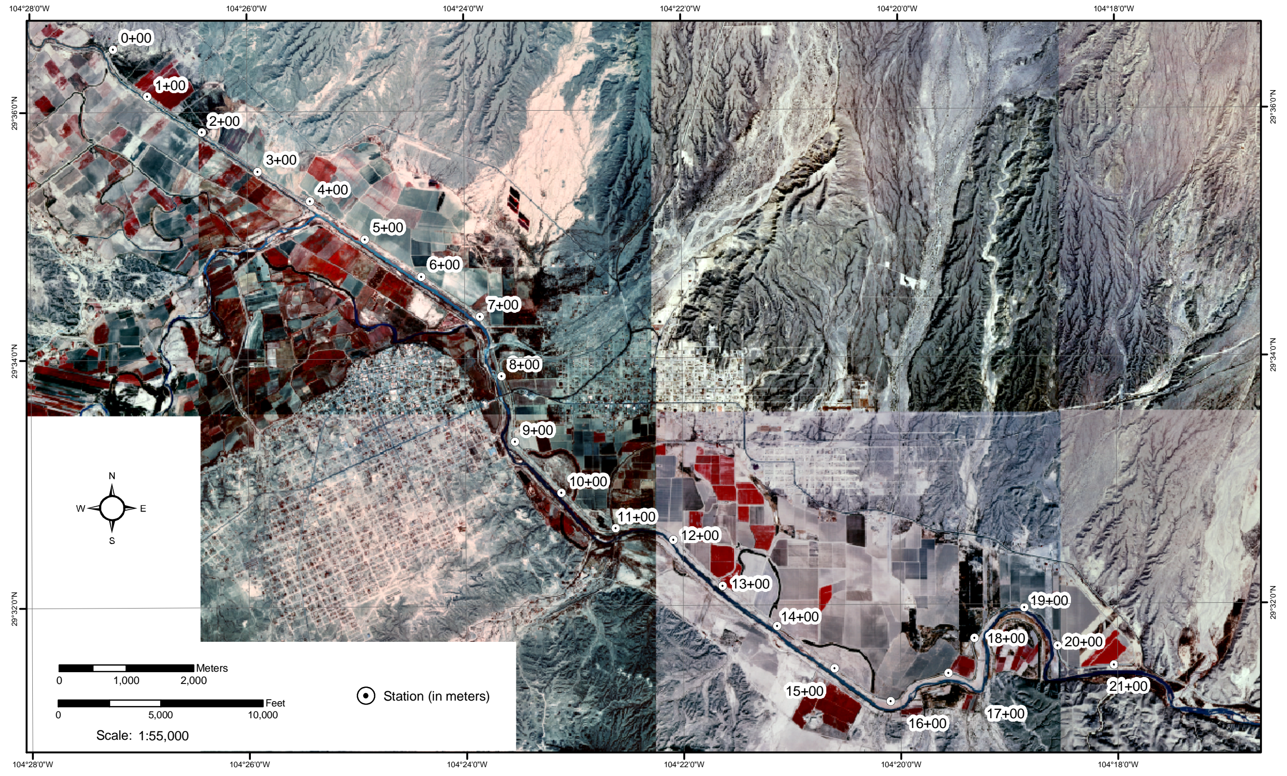
Figure 2. Digital-ortho-quarter-quadrangles (DOQQs) of Presidio levee reach with approximate levee stationing in meters. Levee stationing based on IBWC map from Presidio Project Office.
