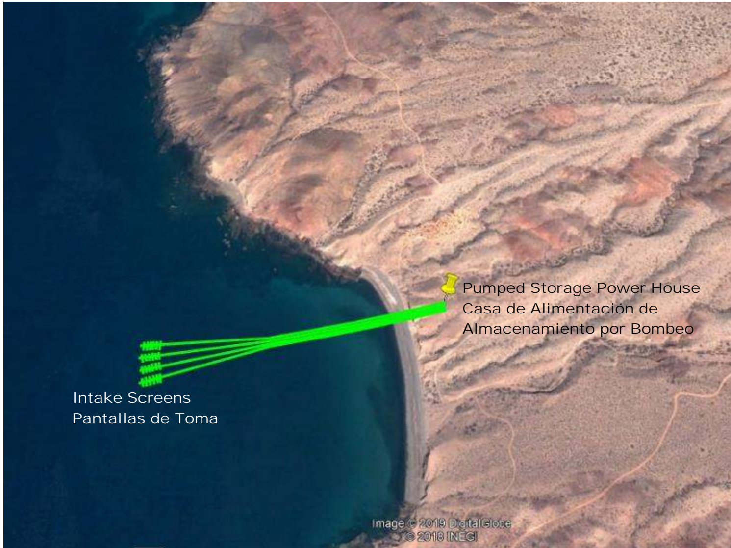
Figure/Figura 27 Opportunity 2 – Marine works plan Opportunidat 2 – Plan de obras marinas
