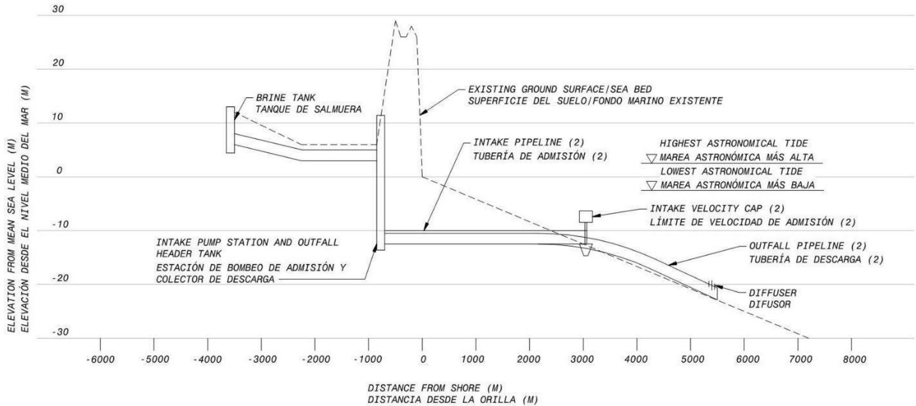
Figure/Figura 10 Opportunity 1 – Marine works profile Opportunida 1 - Perfil de obras marinas
